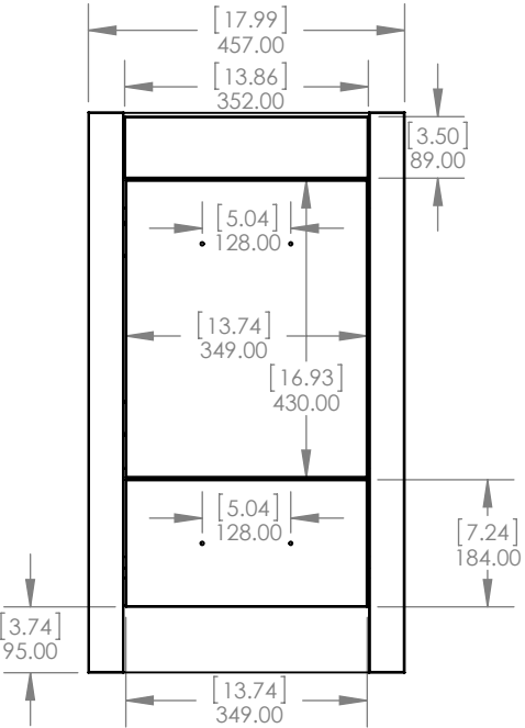
Front view / Vista Frontal
