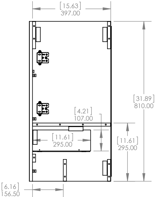
Side View / Vista Lateral
