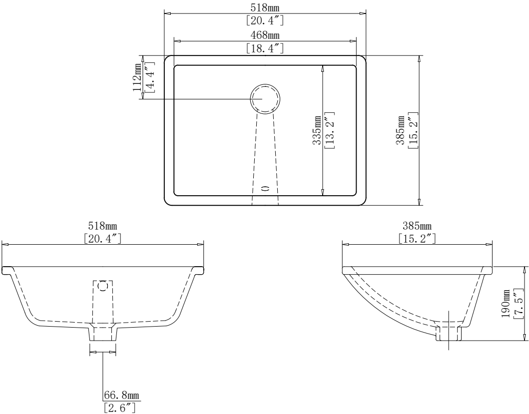
Undermount Sink
