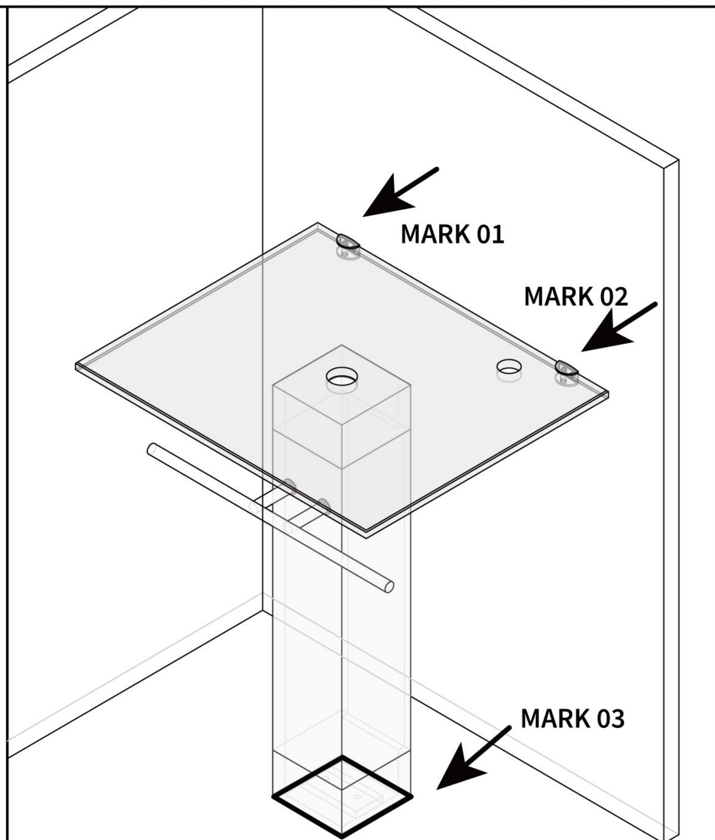
3\ Keep the glass counter top with clips on the pedestal, Make sure the drain hole on the glass countertop are aligned with the drain hole on the pedestal. Then mark the location of the clips on the wall and pedestal on the floor
