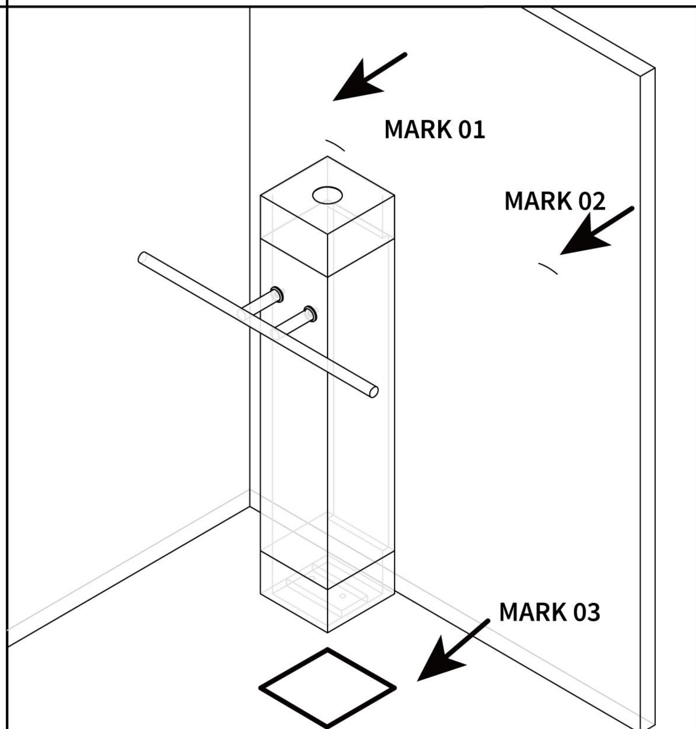
3\ Keep the glass counter top with clips on the pedestal, Make sure the drain hole on the glass countertop are aligned with the drain hole on the pedestal. Then mark the location of the clips on the wall and pedestal on the floor
