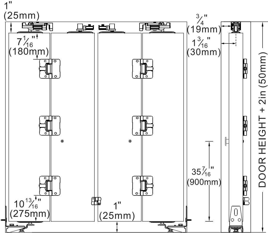
Back view
