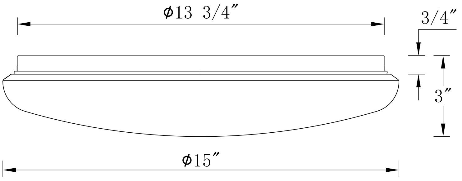
FRONT VIEW
