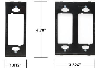
One Gang Plastic Subplate
