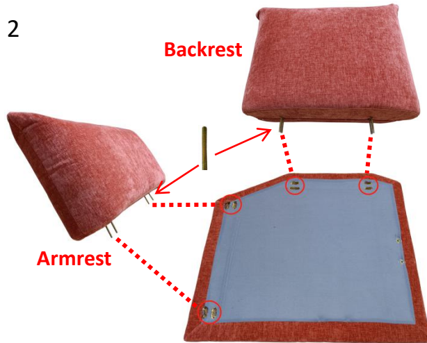
Connecting piece
