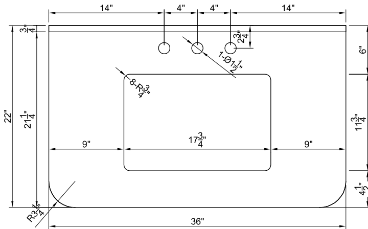
TOP VIEW OF VANITY CABINET
