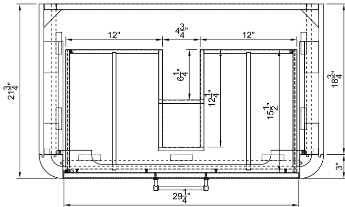
TOP VIEW OF VANITY CABINET
