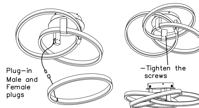
Plug-in Male and Female plugs
