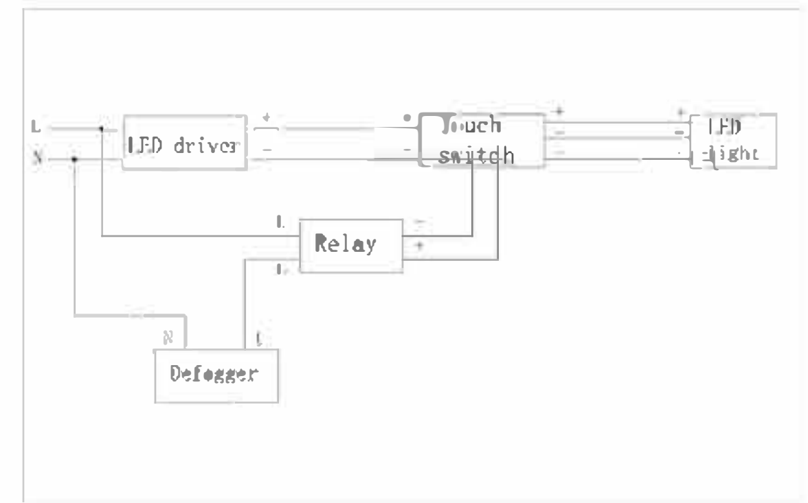
Circuit diagram
