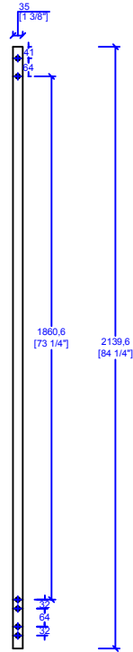
SECTION B-B
