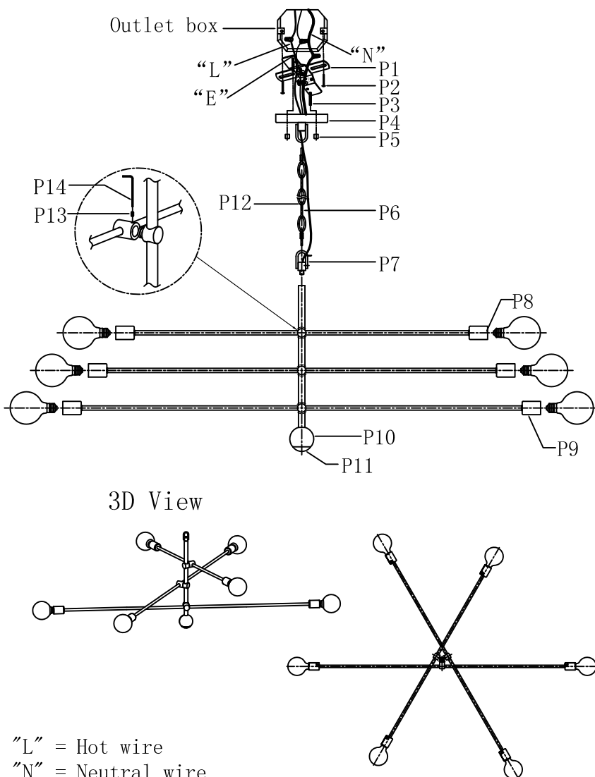
Bottom View 1:4
