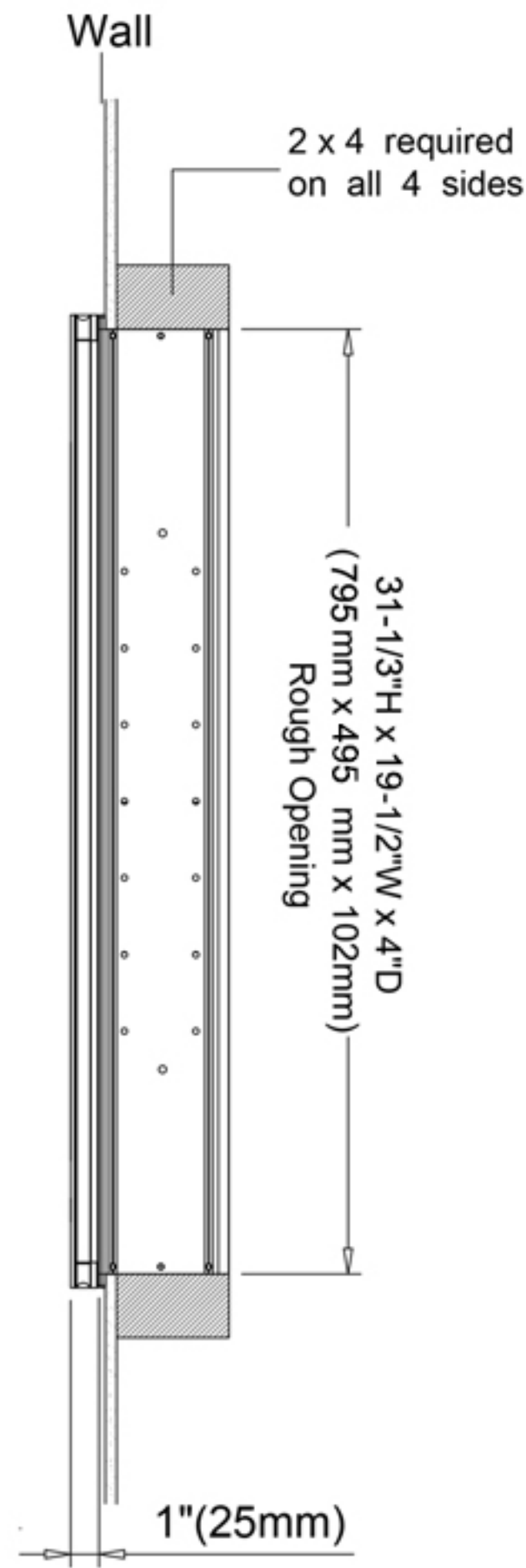
Recessed Mount
