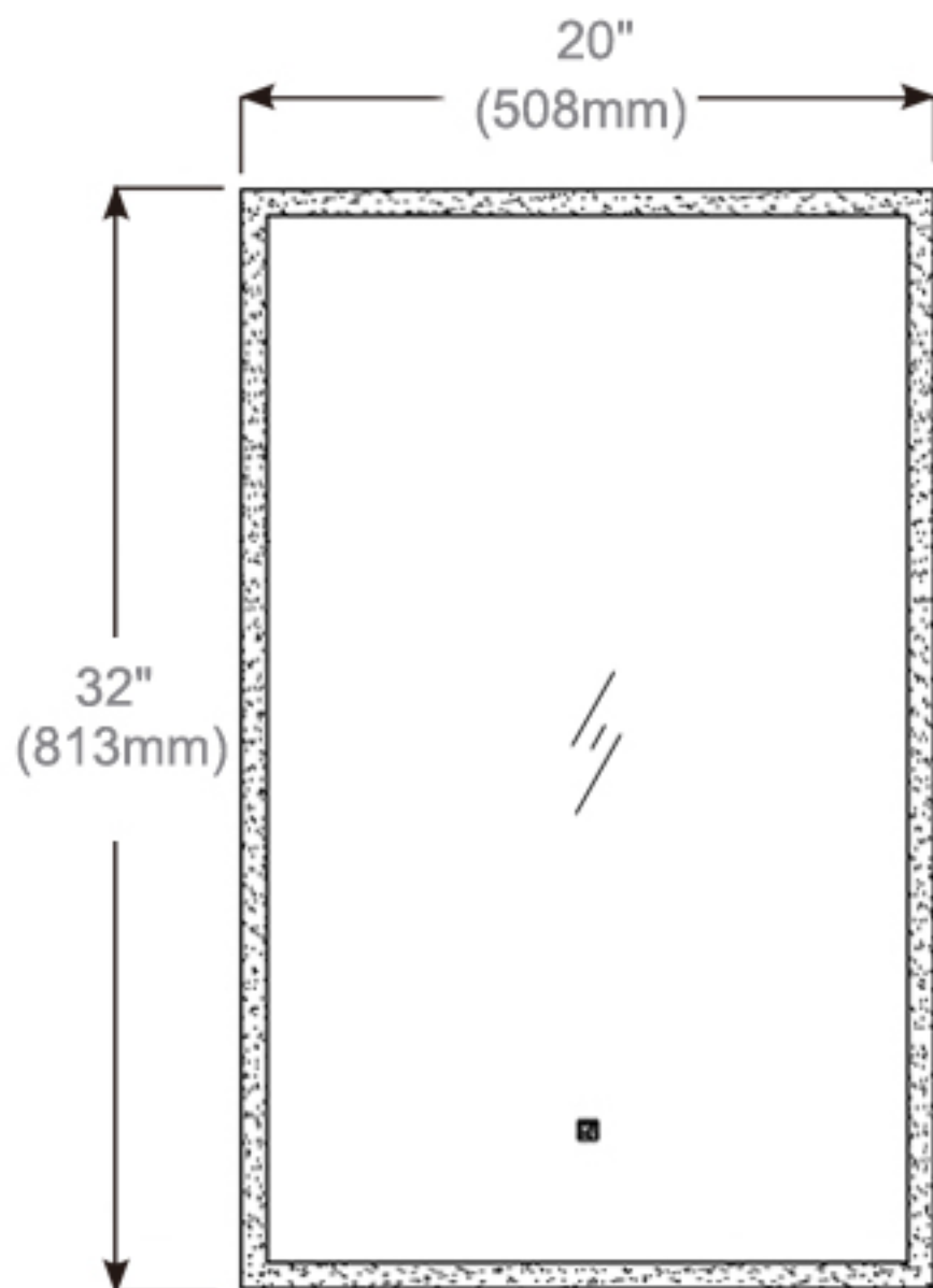
Cabinet Dimensions
