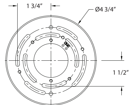
Back Plate Dimensions
