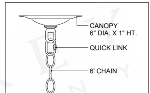
CANOPY DETAIL
