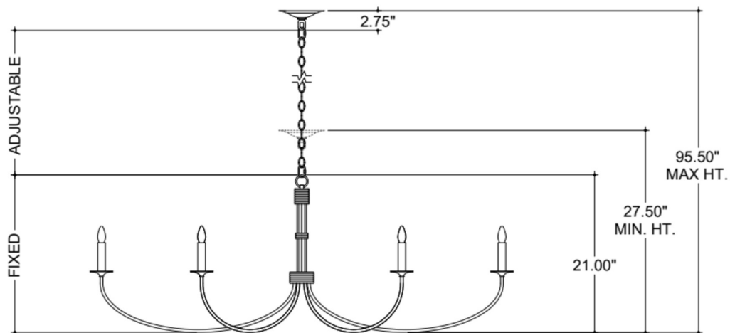
FRONT VIEW
