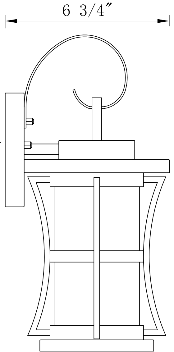
SIDE VIEW
