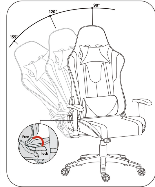
Backrest Adjustment
