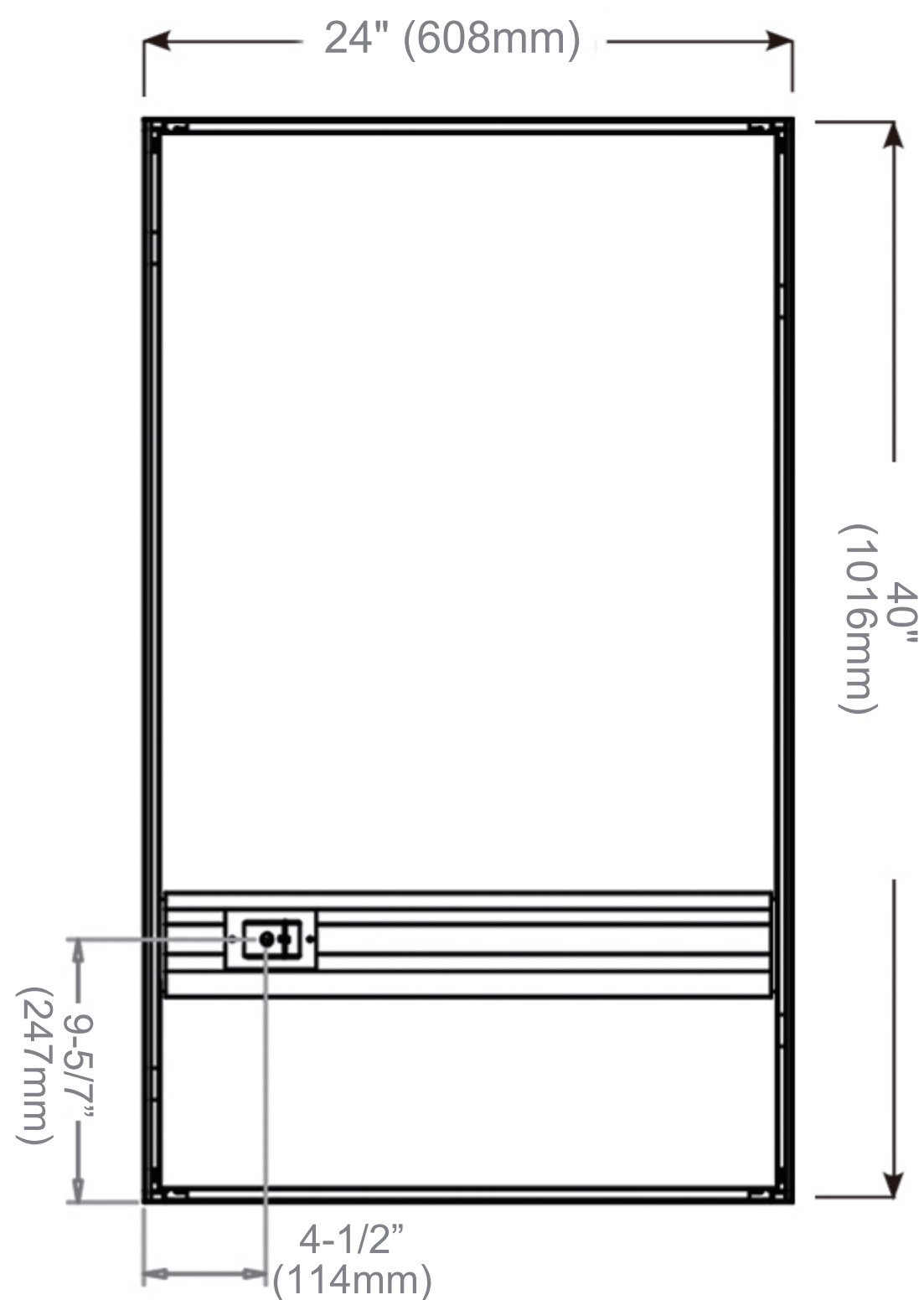
Back of Cabinet - Wire Access Location
