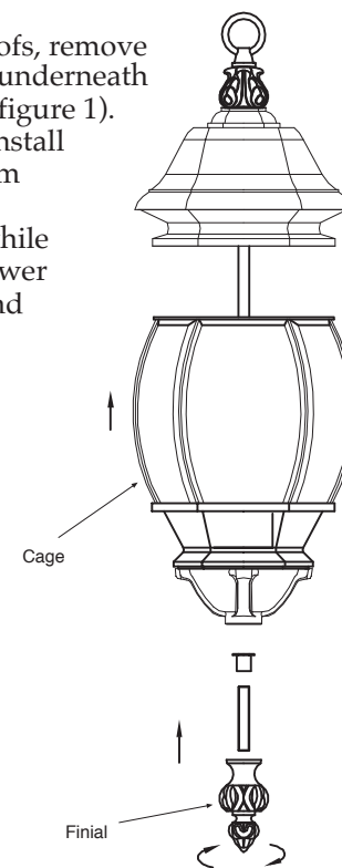
Figure 3 Finial Bottom
