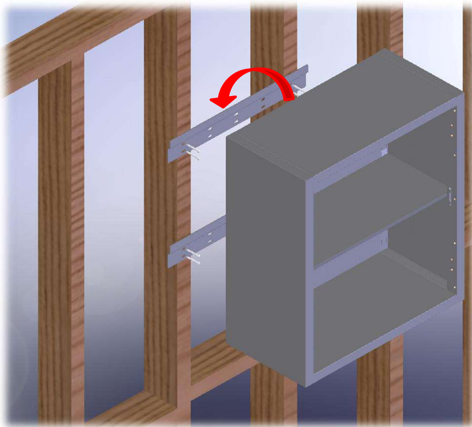
Hang Wall Cabinet Wall-Hanging Brackets
