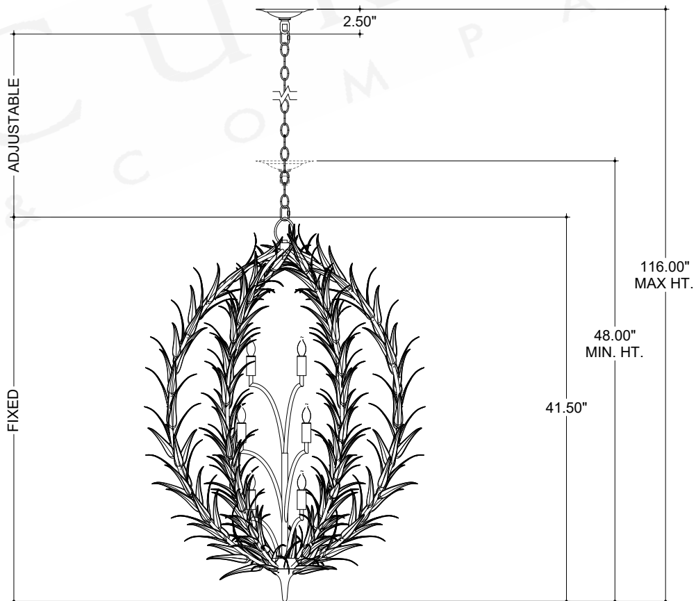
FRONT VIEW
