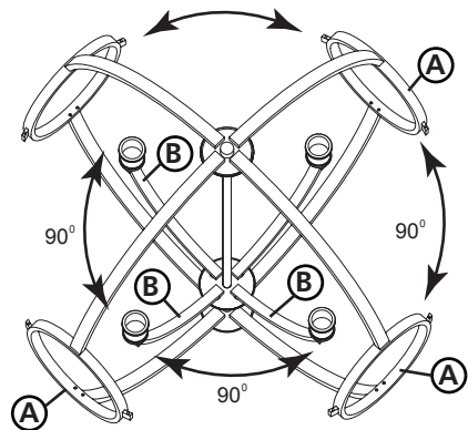
DRAWING 2 - ASSEMBLY
