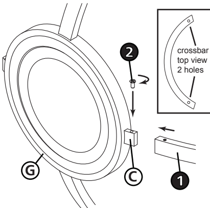
DRAWING 3 - ASSEMBLY
