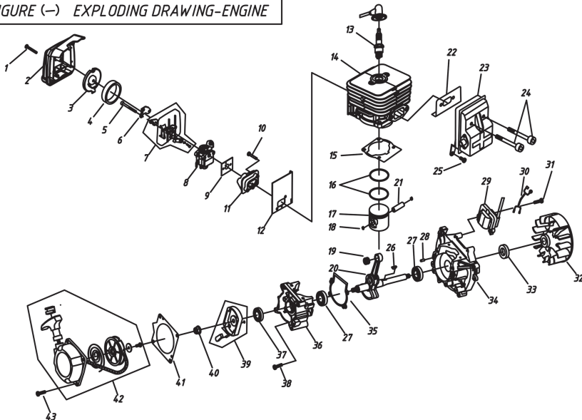
FIGURE (—) EXPLODING DRAWING-ENGINE
