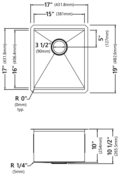
Model #: KWU111-17 Sink Dimensions: 17" x 19" x 10" Min Cabinet Size: 21"
