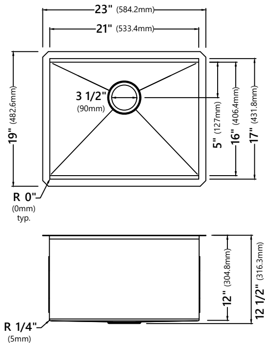
Model #: KWU100-23L Sink Dimensions: 23" x 19" x 12" Min Cabinet Size: 27"
