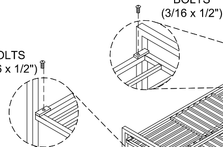
SCREWS (#10 x 3/4")
