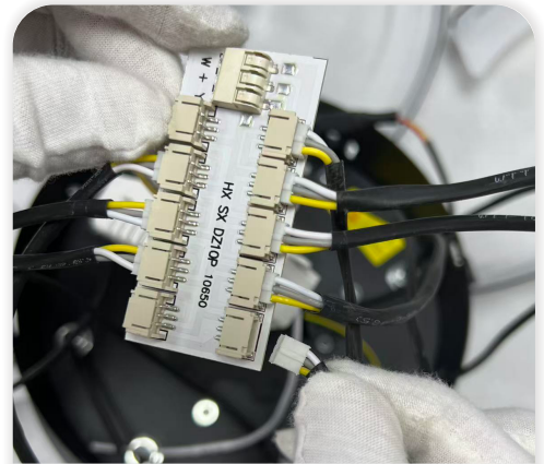
18 Insert the wires of the other lamp holders in sequence.
