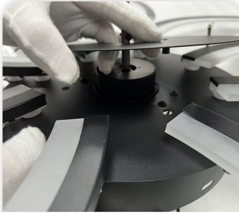
14 Install the circular iron piece.
