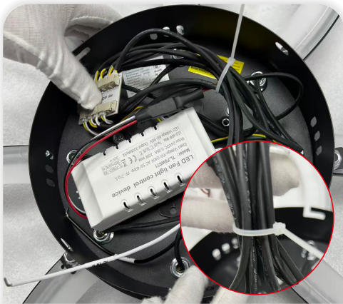
19 Use cable ties to bundle the wires.
