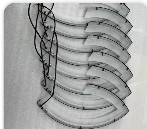
6 Install the other lamp holders in sequence.
