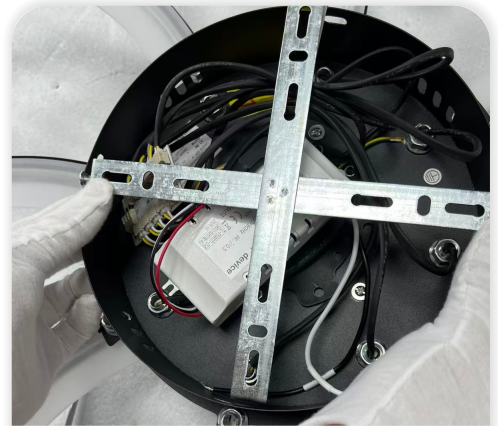
21 Check and tighten the other four screws.
