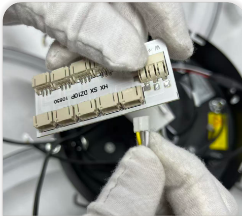
17 Insert the lamp holder wire into the terminal block.
