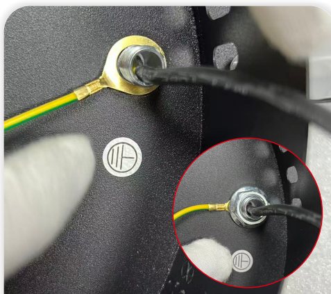
11 Insert the ground wire into the lamp holder wire and tighten with a screw
