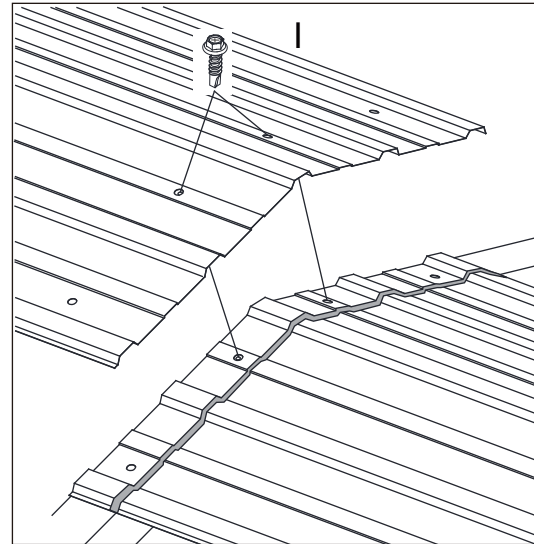
Assembly sequence for the roof sheet
