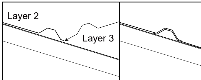
Assembly sequence for the roof sheet
