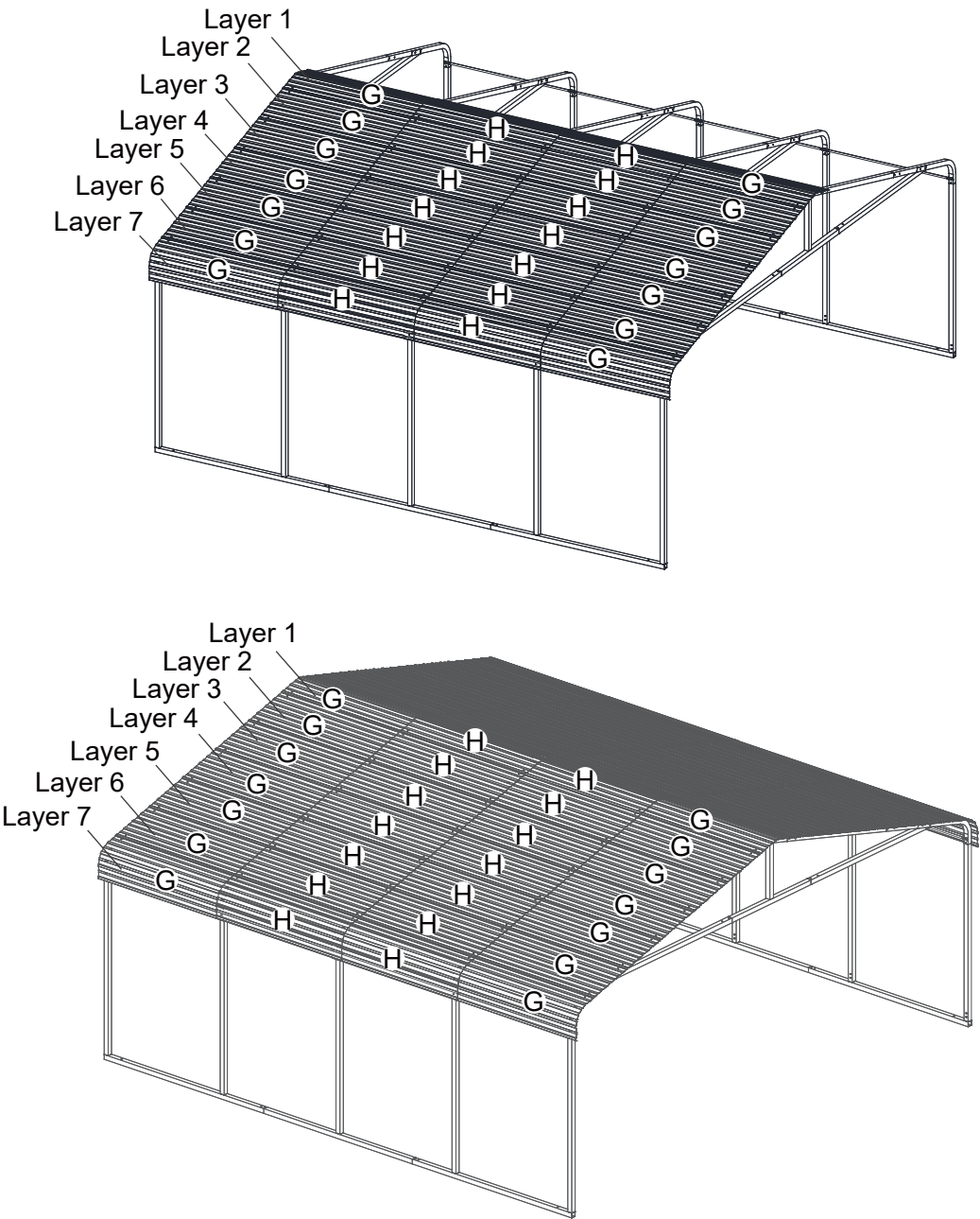
Assembly sequence for the roof sheet
