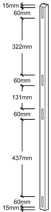
Mirror Support
