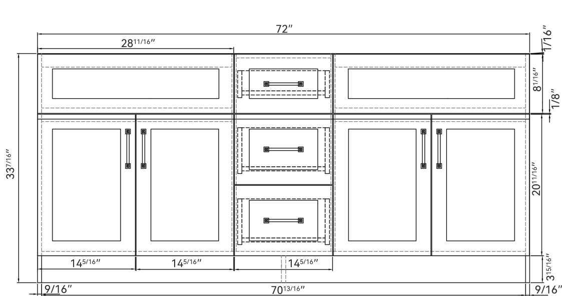
Front View
