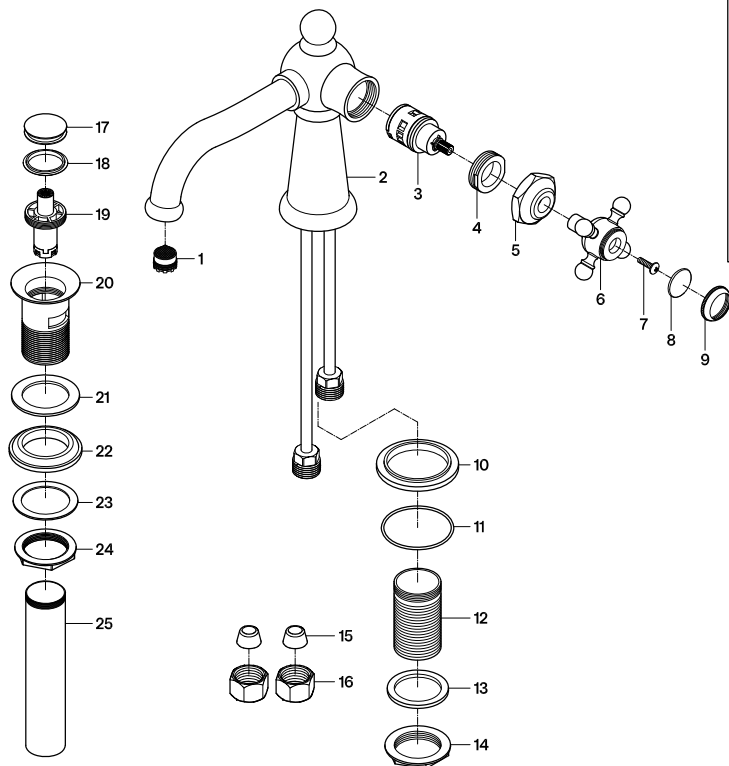
Cartridge: KSRP154C
