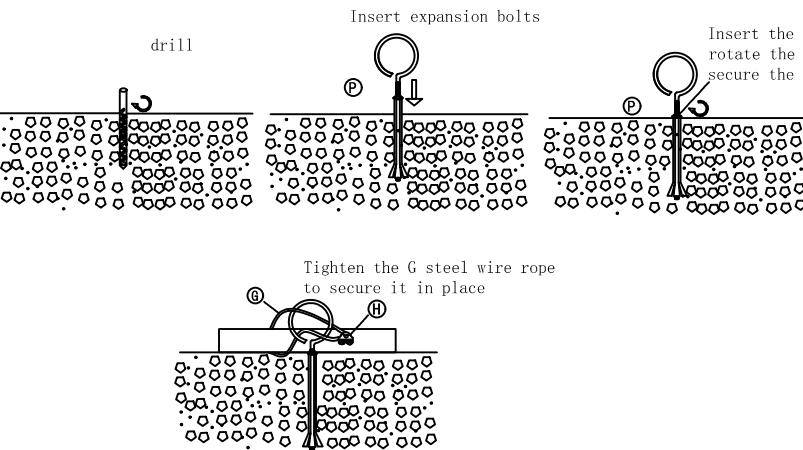
hard ground
