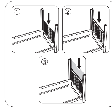
Install Ventilation Meshes and Side Glasses (Left and Right side)
