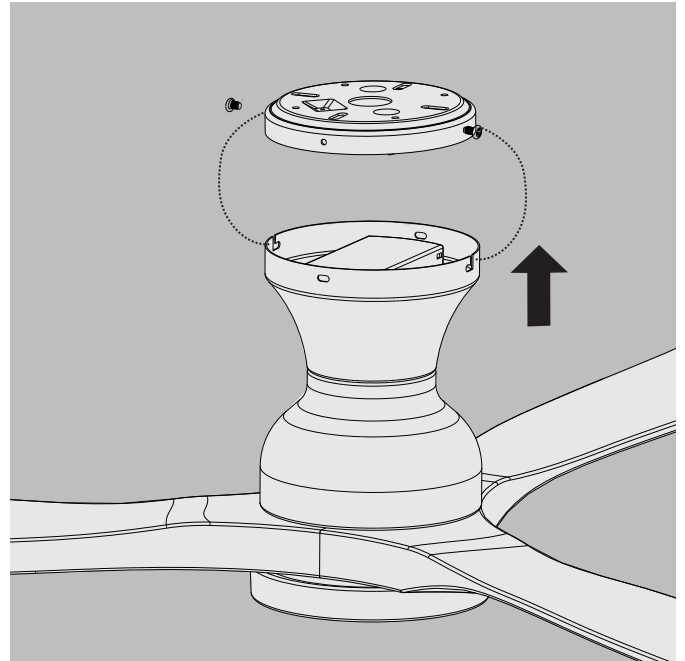
② Insert the ceiling fan into the gap position
