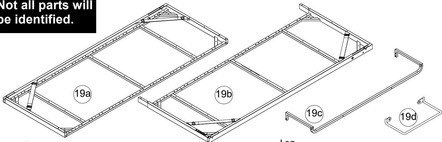
Right Assembly 9632096-19b
