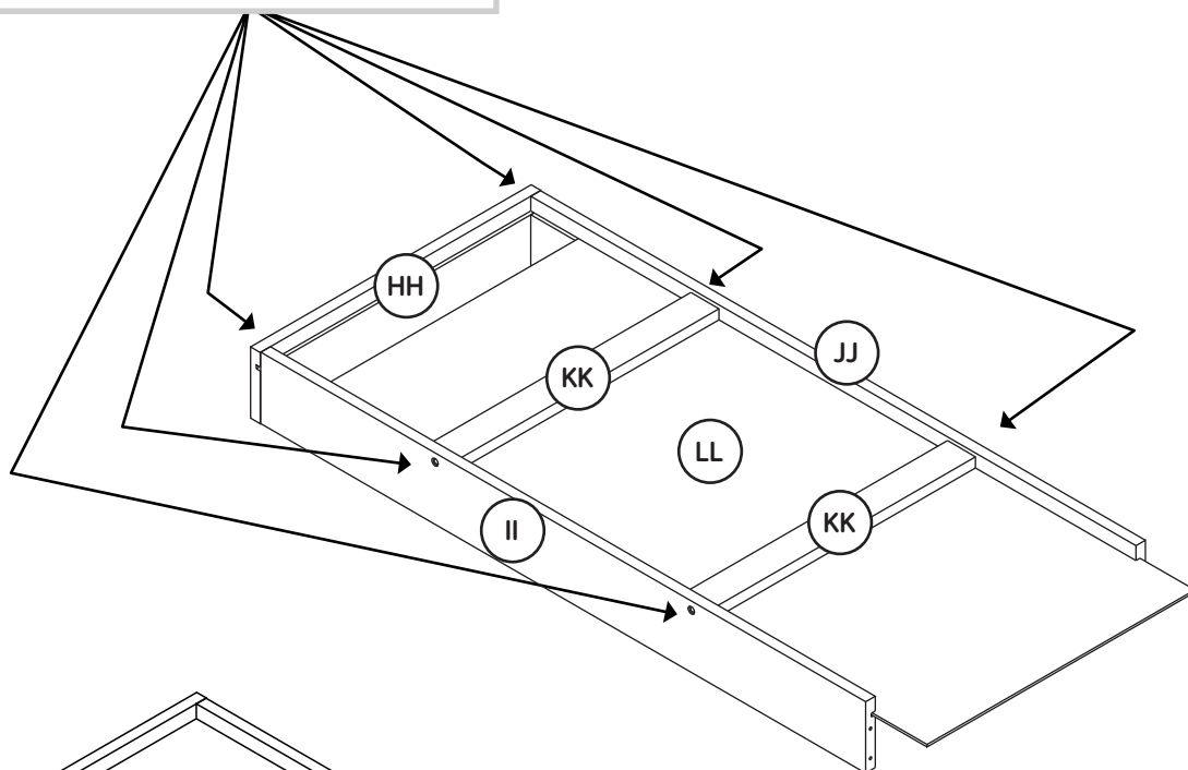
BLACK 1-9/16" FLAT HEAD SCREW (12 used in this step)
