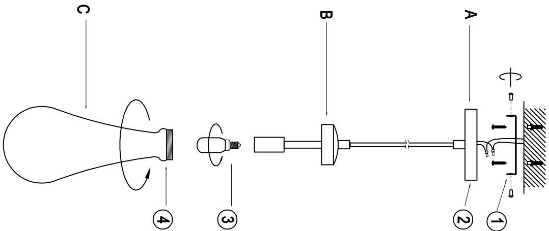
Installation sequence diagram
