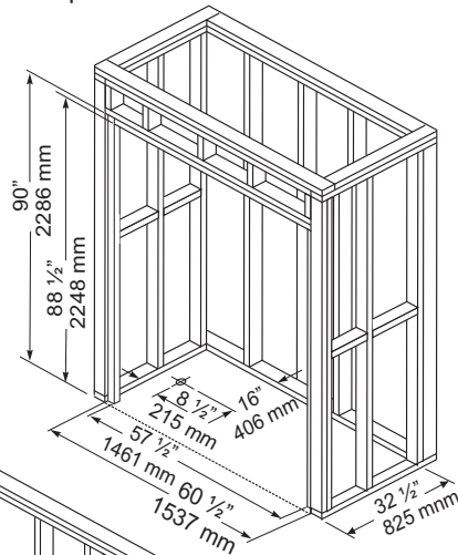
FIGURE 1 - LAYOUT DIMENSIONS
