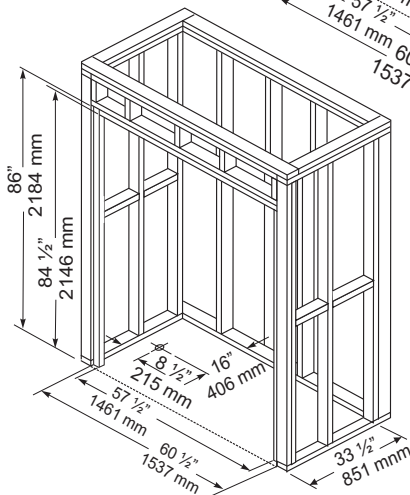
FIGURE 1 - LAYOUT DIMENSIONS
