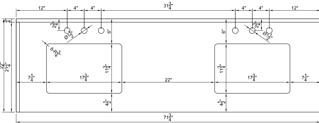
TOP VIEW OF VANITY CABINET
