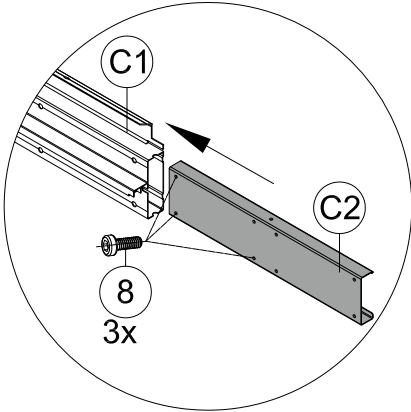
(1) Insert Part #C2 into Part #C1 and secure with 3 Bolts #8.
