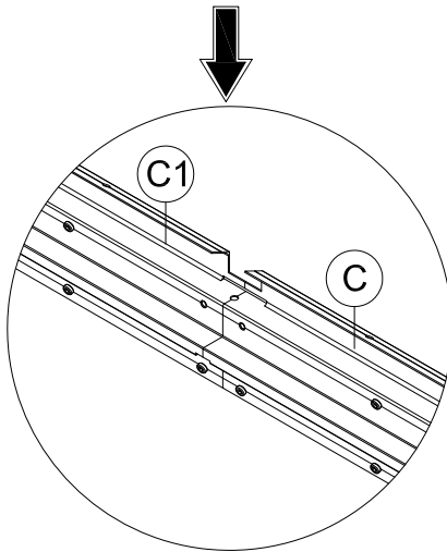
(4) Insert Part #X into the beam and secure with 1 Bolt #8.
