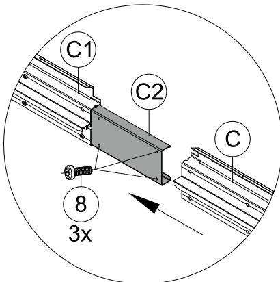
(2) Insert the other side of Part #C2 into Part #C and secure with 3 Bolts #8.
