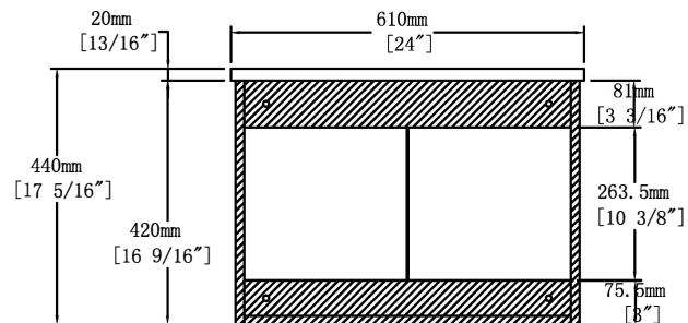
Back View
