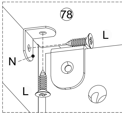
Left x2
