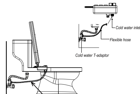
7. Connect cold water supply to bidet
