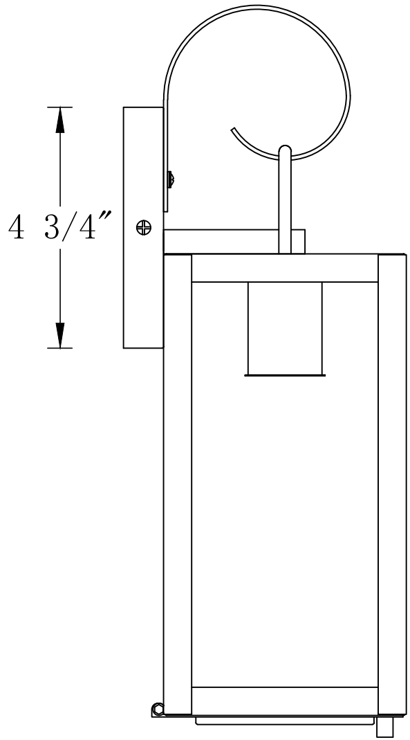
SIDE VIEW
