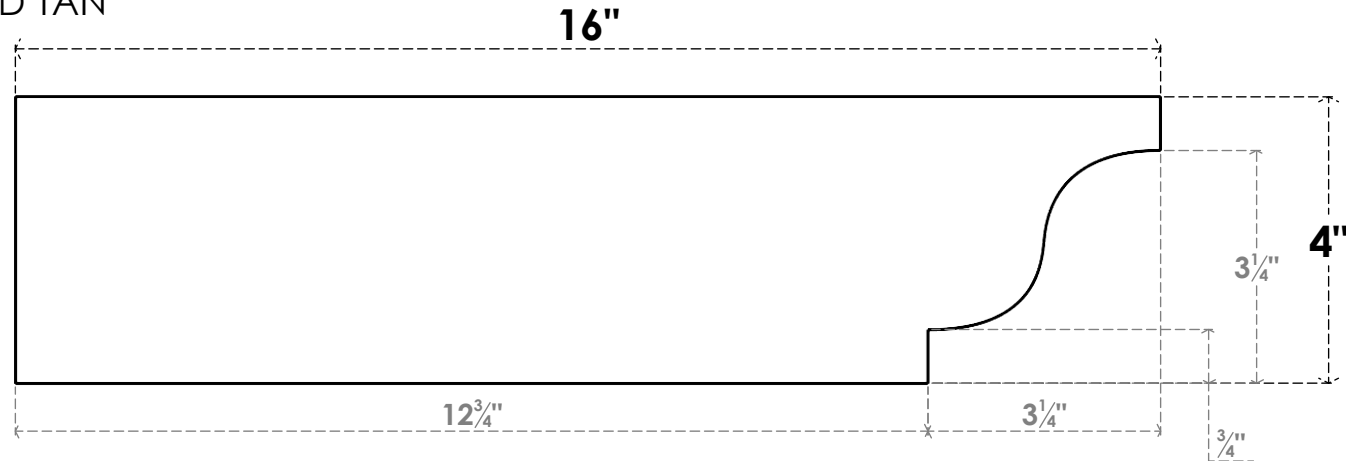
SIDE PROFILE
