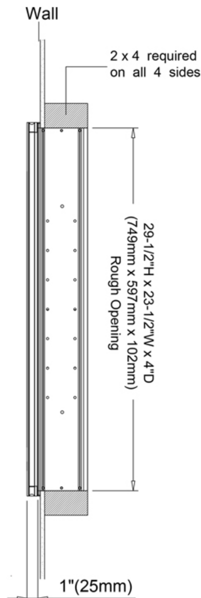
Recessed Mount
