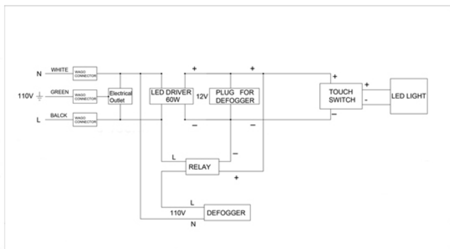
Circuit Diagram
