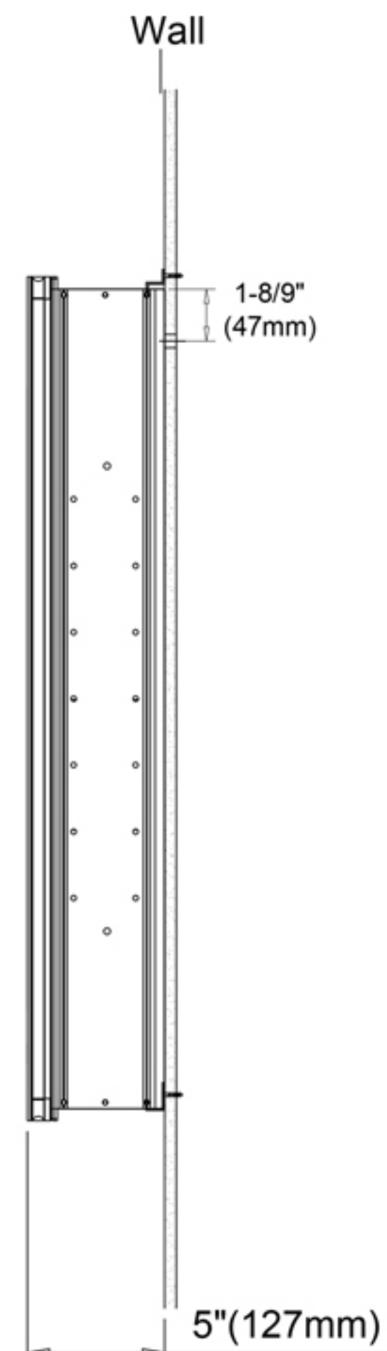
Surface Mount
