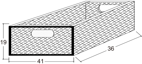
DETAIL BASKET
