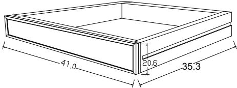
DETAIL DRAWER
