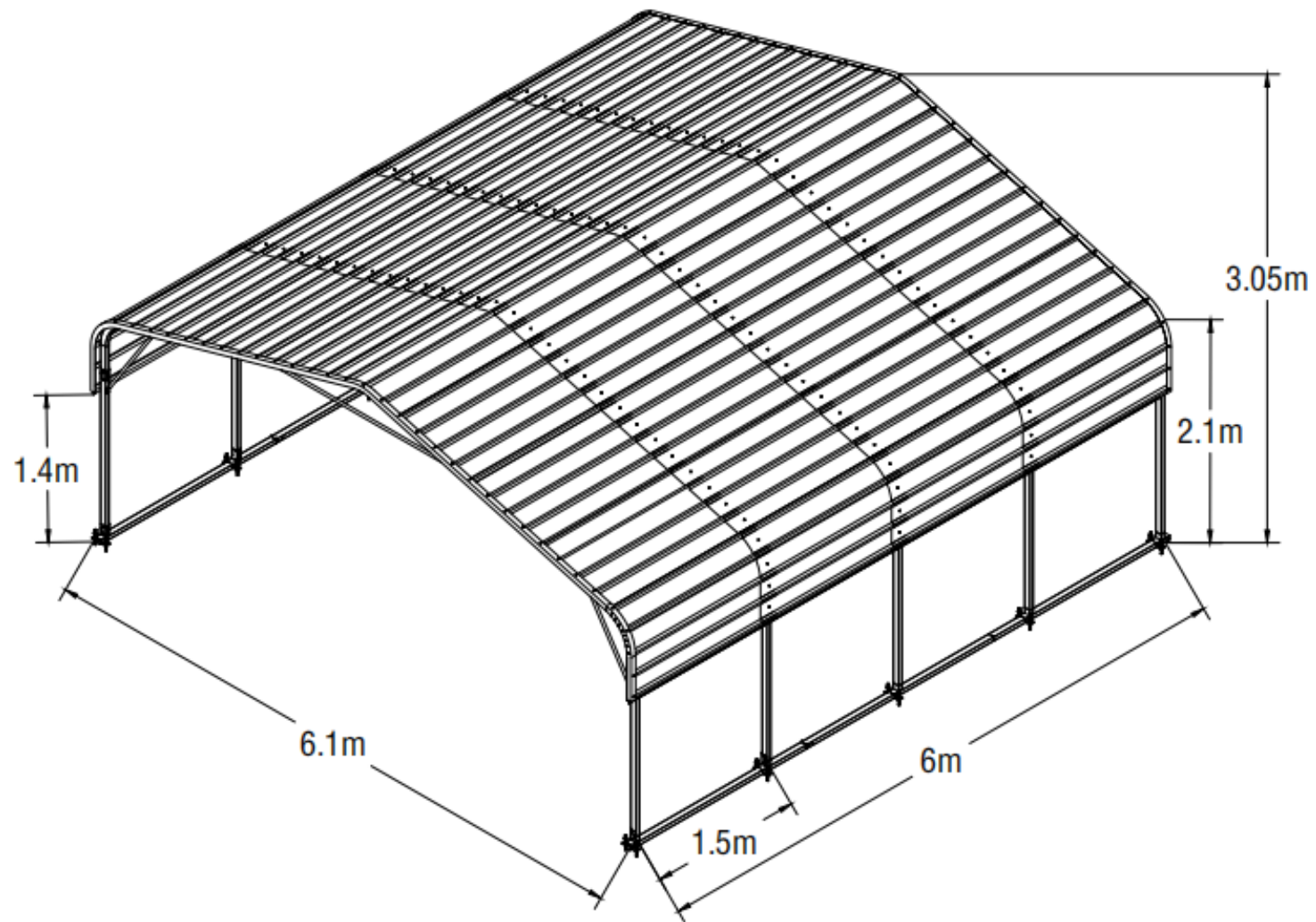
Frame Sketch 2
