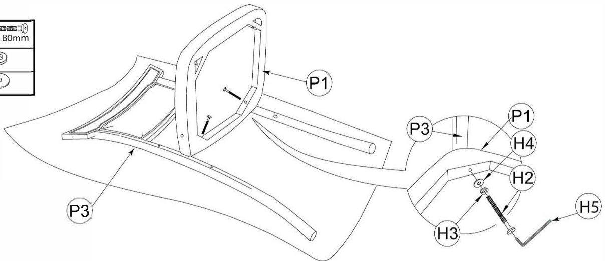
COMPLETE ASSEMBLY
