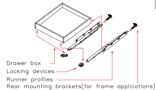
Full extension concealed drawer runners
