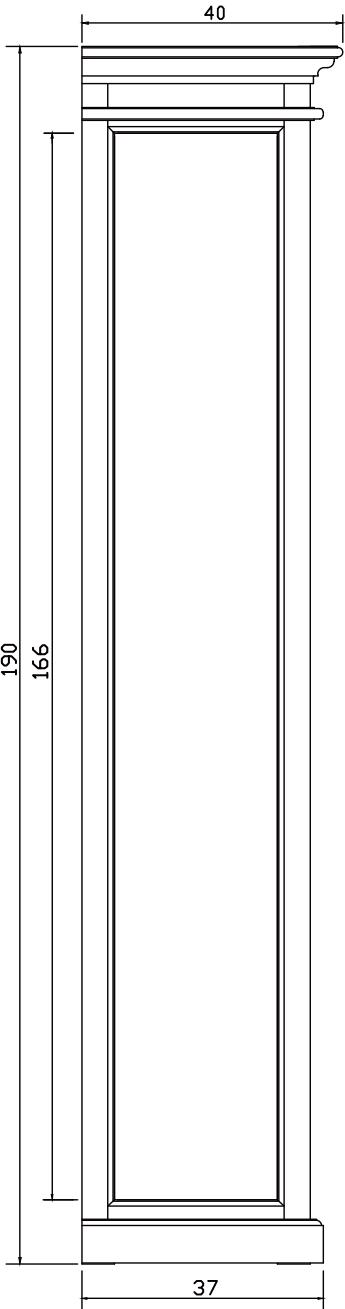
SIDE VIEW
