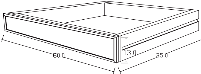
DETAIL DRAWER
