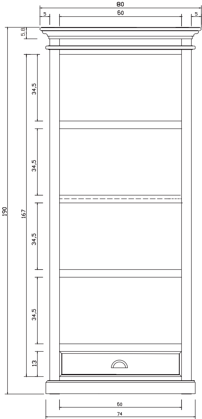
FRONT VIEW
